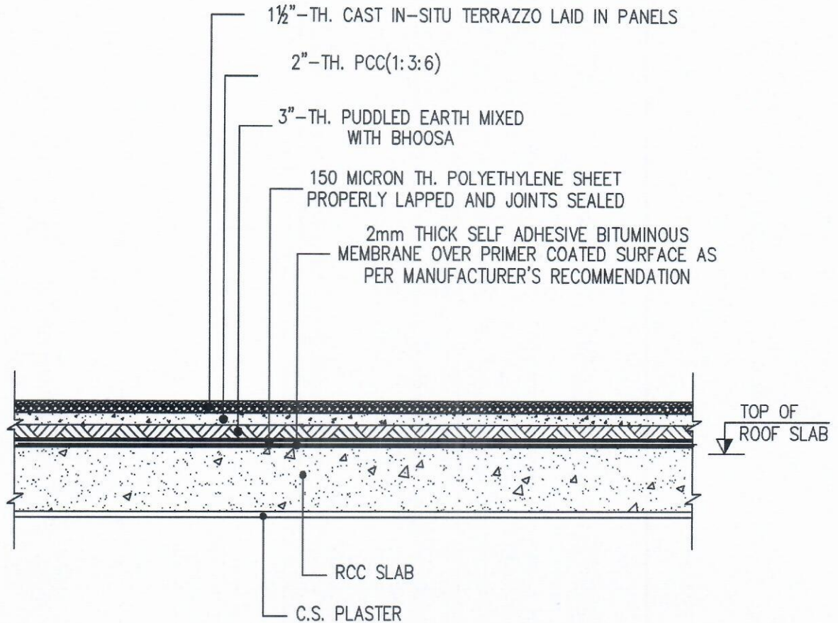
TYPICAL DETAIL OF ROOF TREATMENT
